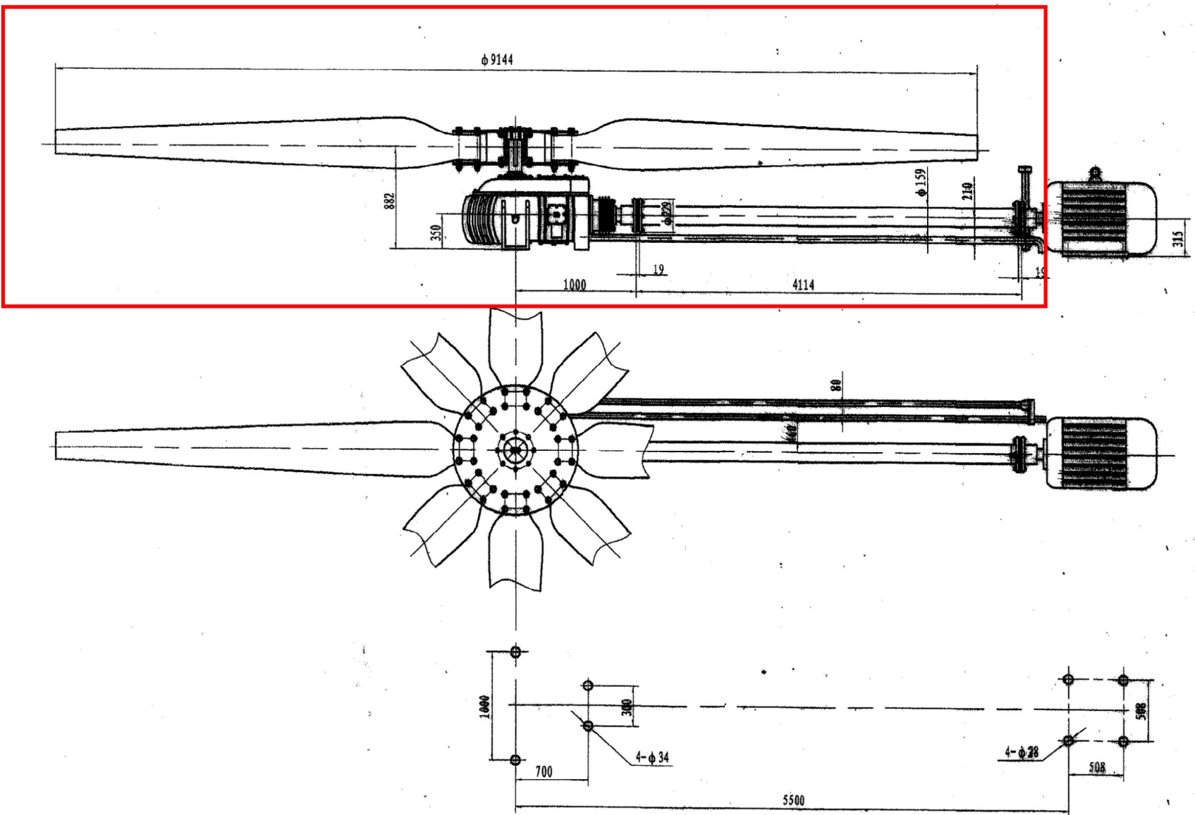
Figure 1 Assembly dimension figure of LF-92 I EZ 6 type fan
