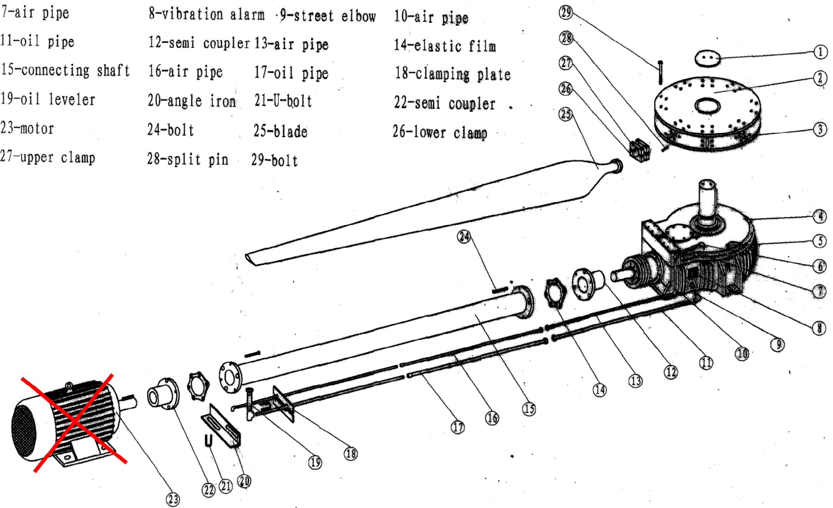
Figure 5 General assembly figure of the fan with single shaft
